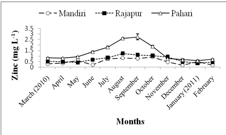
Figure 4 Monthly variation of Zn ( \text{mg L}^{-1} ) of sewage water at three sites viz. Mandiri, Rajapur and Pahari from March 2010 to February 2011. The values are means of respective three replicates with standard errors as vertical error bars.
